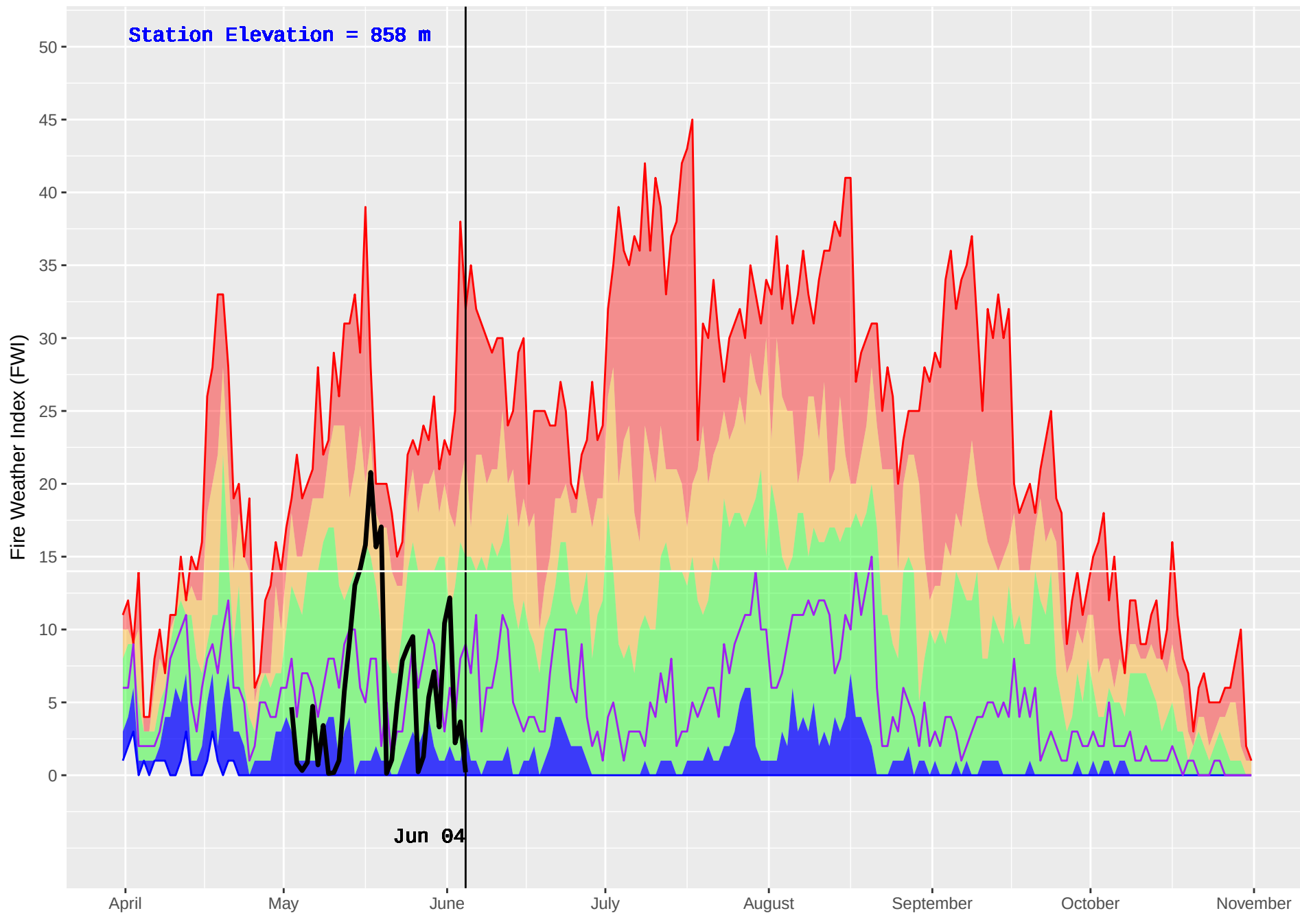
BEDNESTI (175) : Historical (1993–2016) and Current (2018) Noon Fire Weather Index (FWI)
